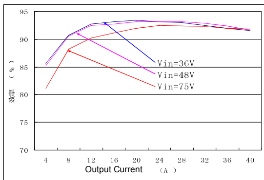
Efficiency vs Output Current (Tc=+25°C)
