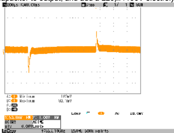
25%-50%-25% I_o Dynamic Load
