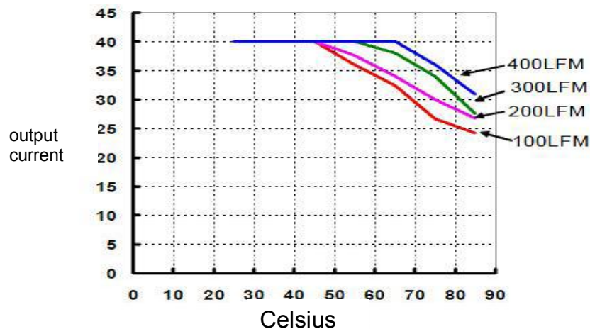
Thermal Derating Curve with no heat sink at different wind speeds (Vinom)
